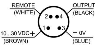
M8 CONNECTOR
